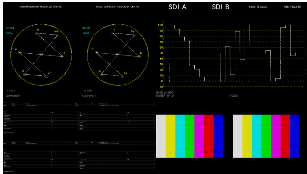
Figure 6-45 Normal display
