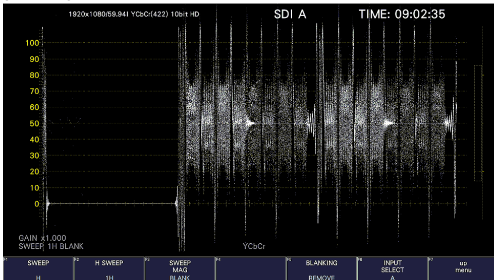
Figure 10-20 Horizontal magnifications
