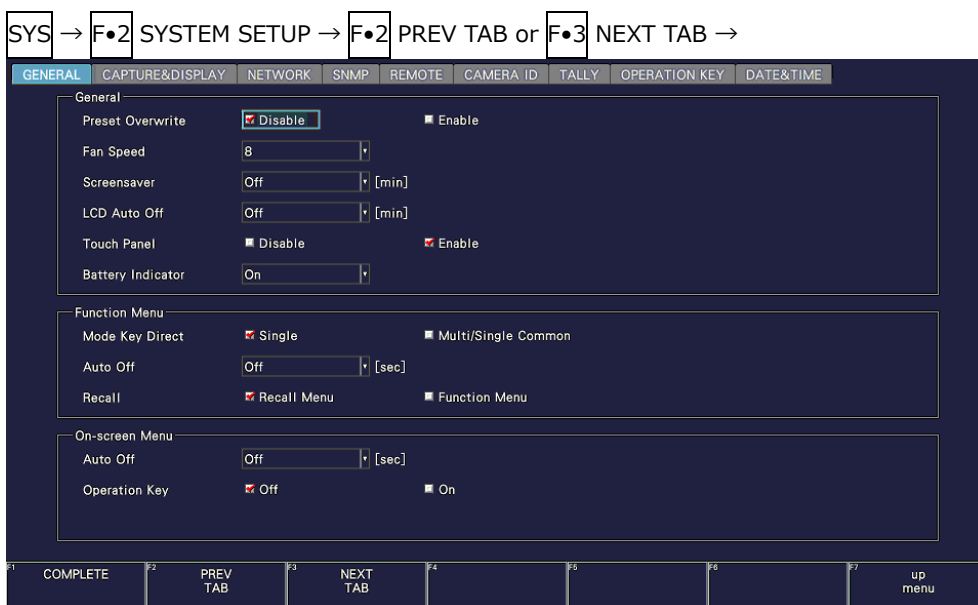
Figure 7-13 GENERAL tab
