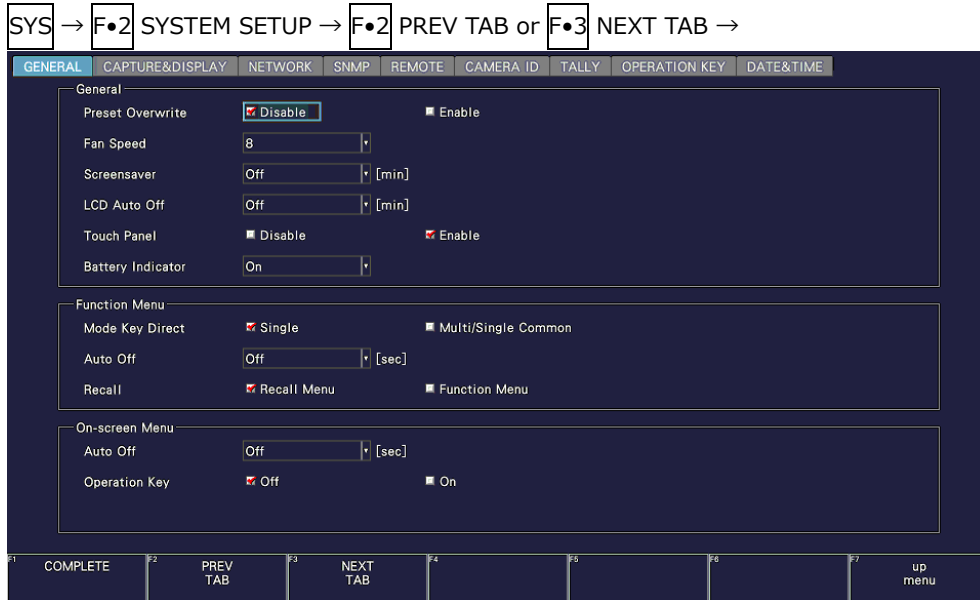
Figure 7-11 GENERAL tab
