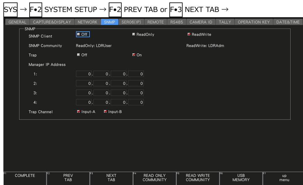
Figure 19-11 SNMP tab
