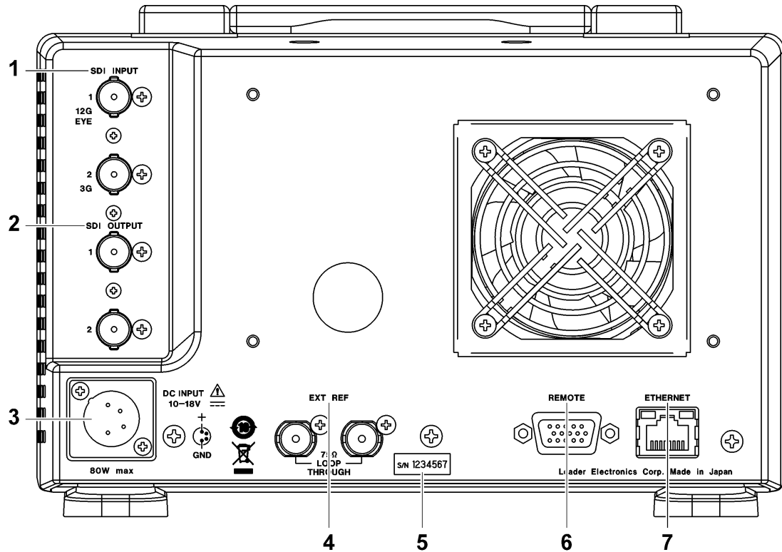
Figure 4-4 LV5300/LV5300A rear panel
