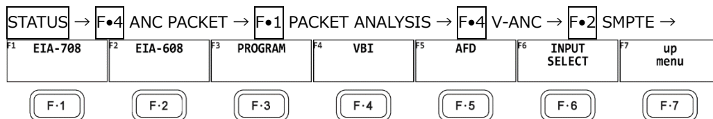
Figure 16-30 SMPTE menu
