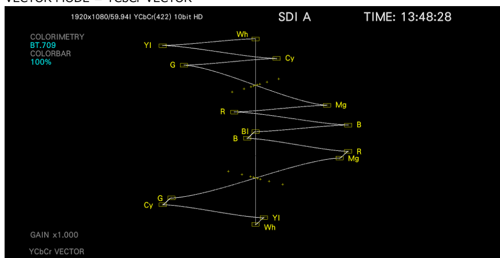
Figure 11-3 Vector mode
