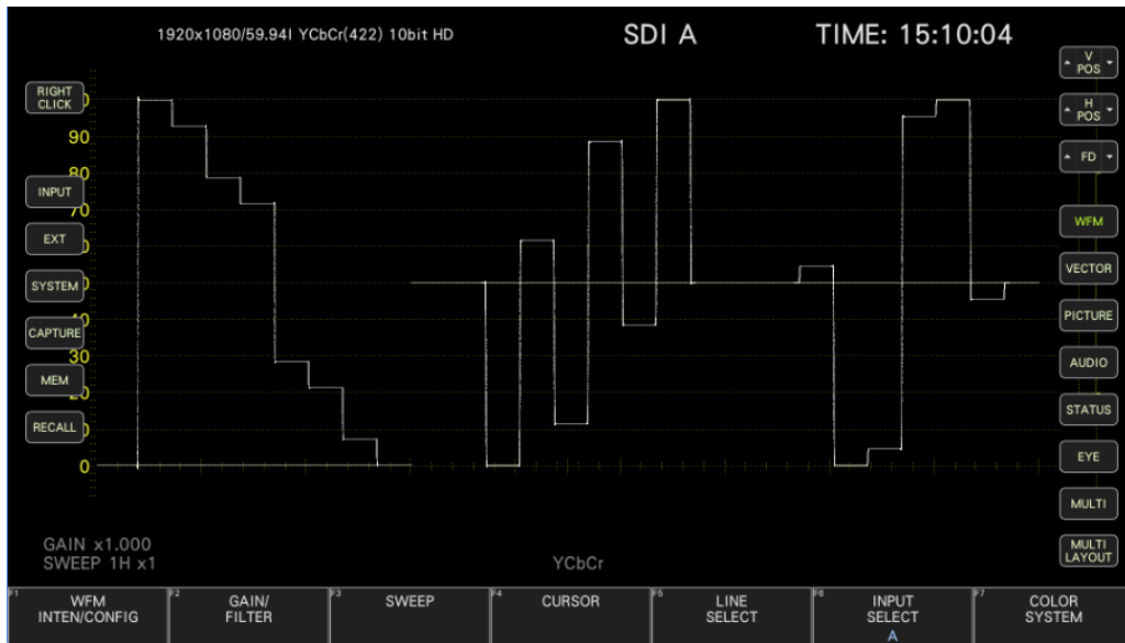
Figure 19-8 DISPLAY
