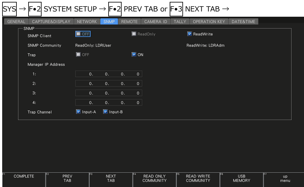
Figure 7-19 SNMP tab
