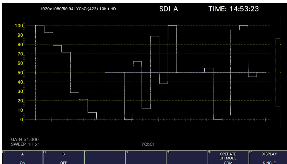
Figure 6-8 Measurement screen
