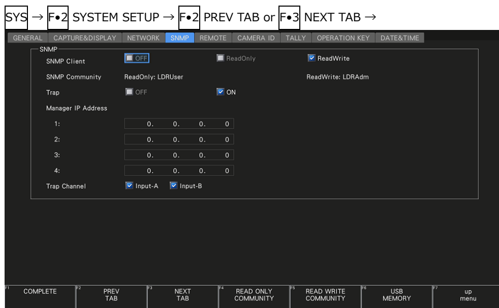
Figure 19-11 SNMP tab
