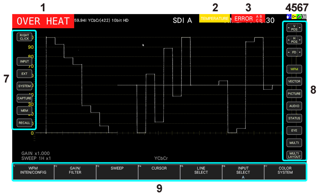
Figure 5-16 Measurement screen description
