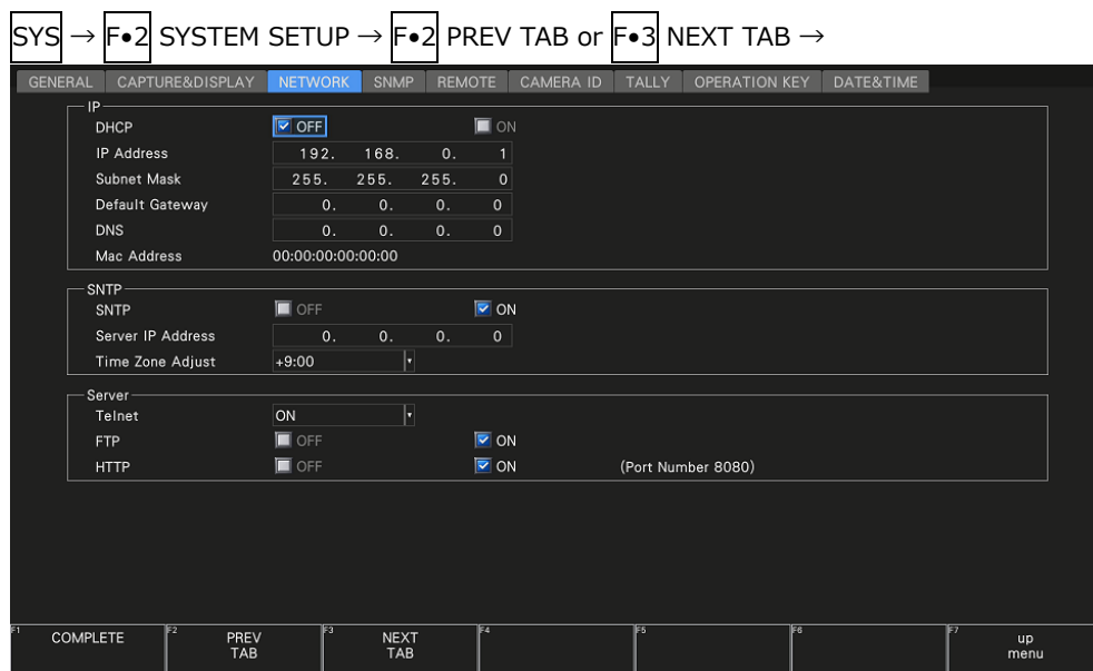
Figure 7-17 NETWORK tab
