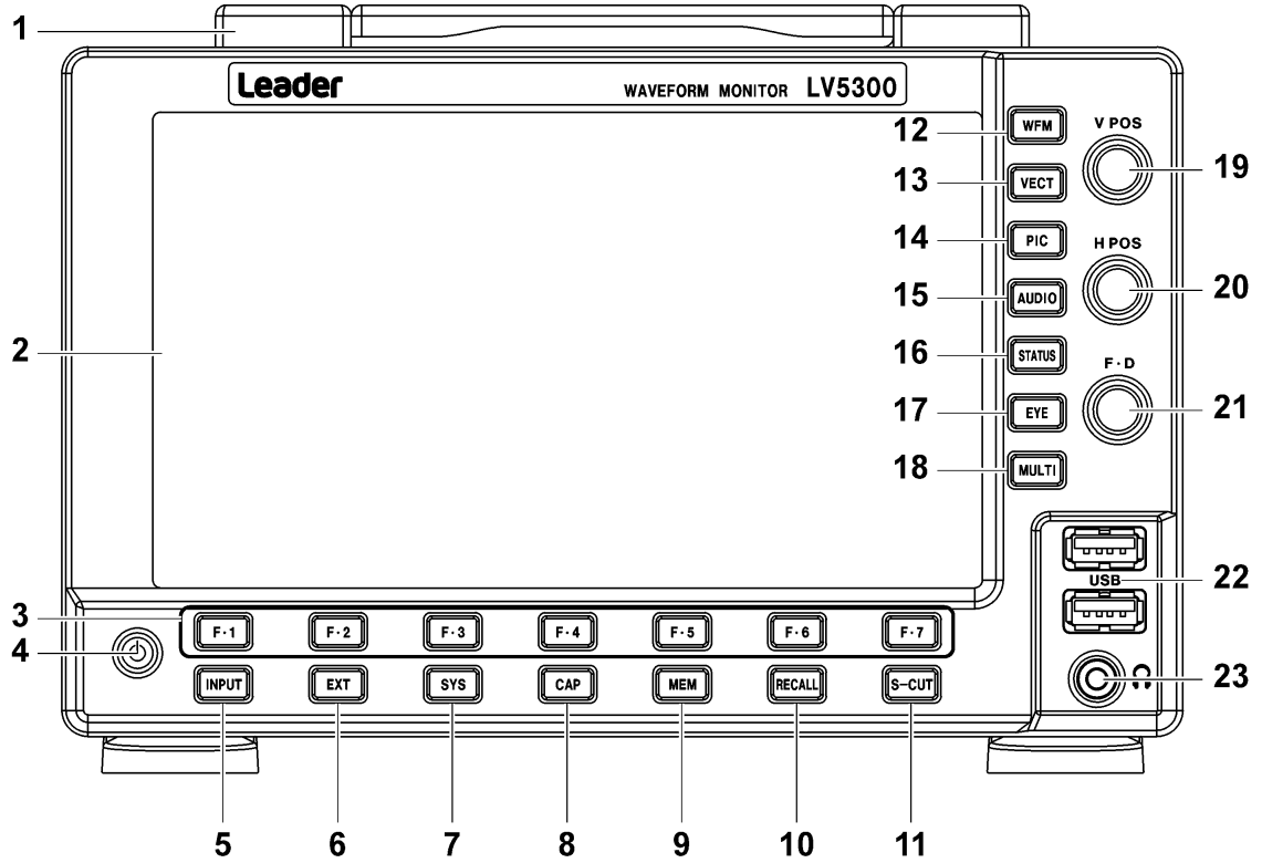
Figure 4-1 LV5300/LV5300A front panel
