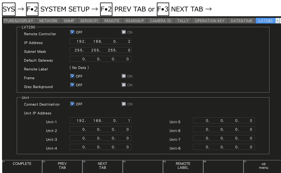
Figure 7-28 LV7290 tab
