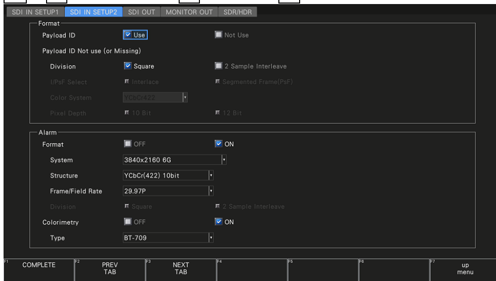
Figure 6-10 SDI IN SETUP2 tab
