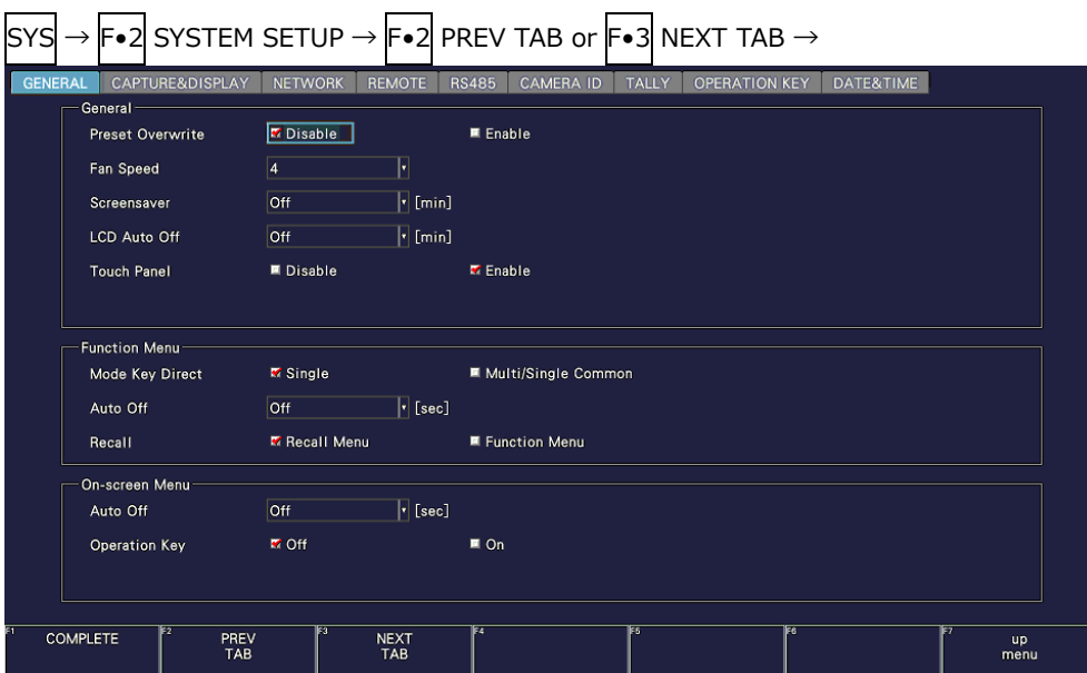
Figure 7-28 GENERAL tab
