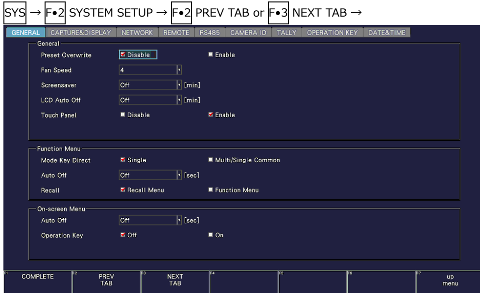
Figure 7-26 GENERAL tab
