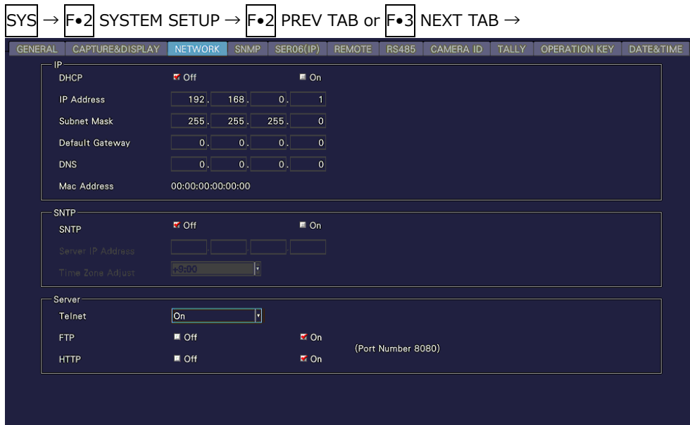
Figure 7-33 NETWORK tab
