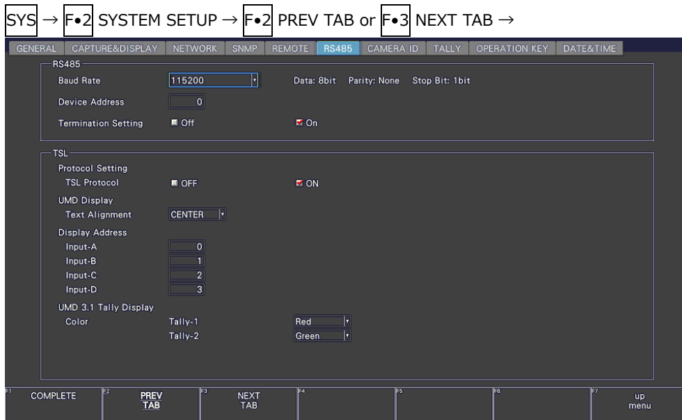
Figure 7-39 RS485 tab
