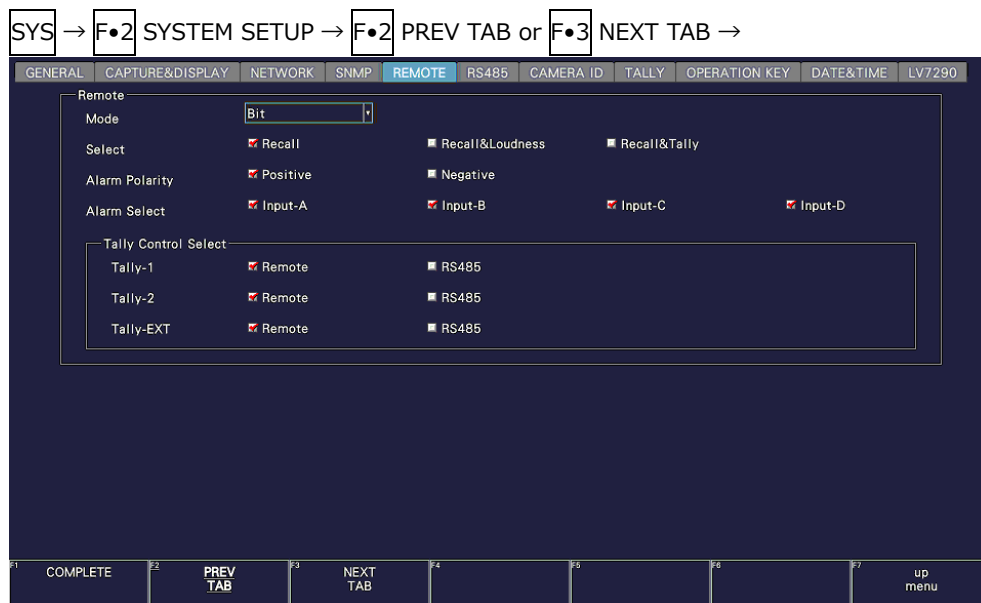
Figure 7-38 REMOTE tab
