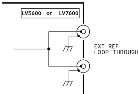
Figure 5-4 Loop-through
