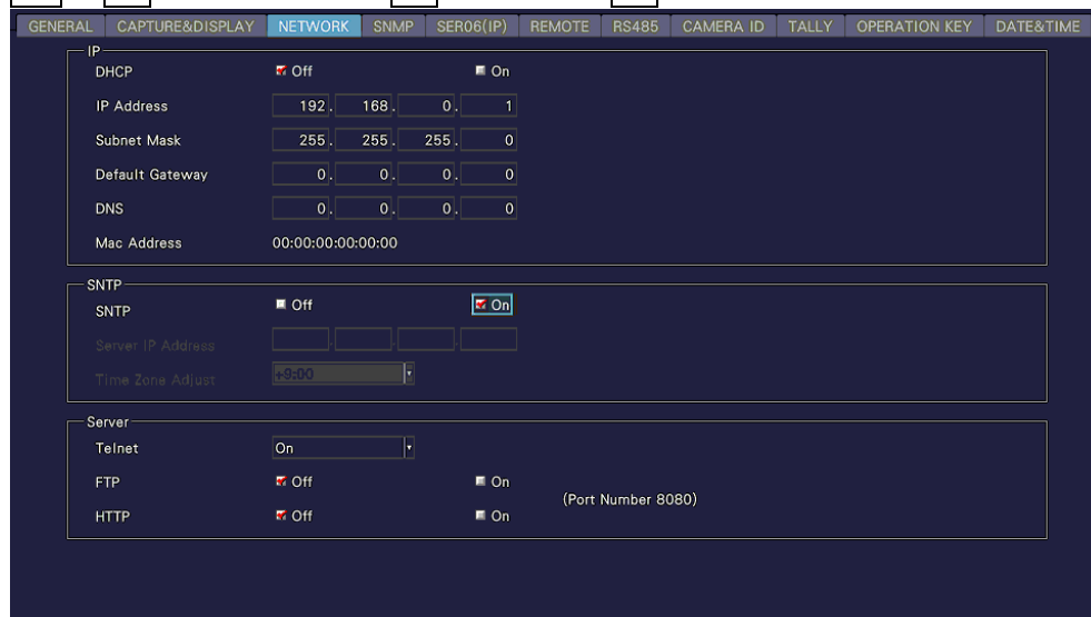
Figure 7-32 NETWORK tab
