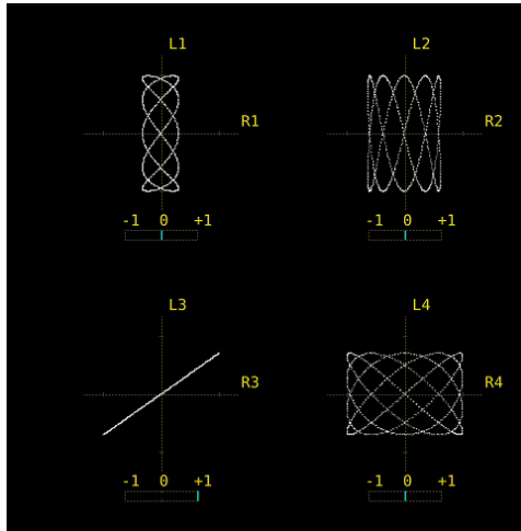
Figure 15-21 Setting the Lissajous curve gain
