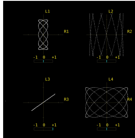
Figure 15-21 Setting the Lissajous curve gain
