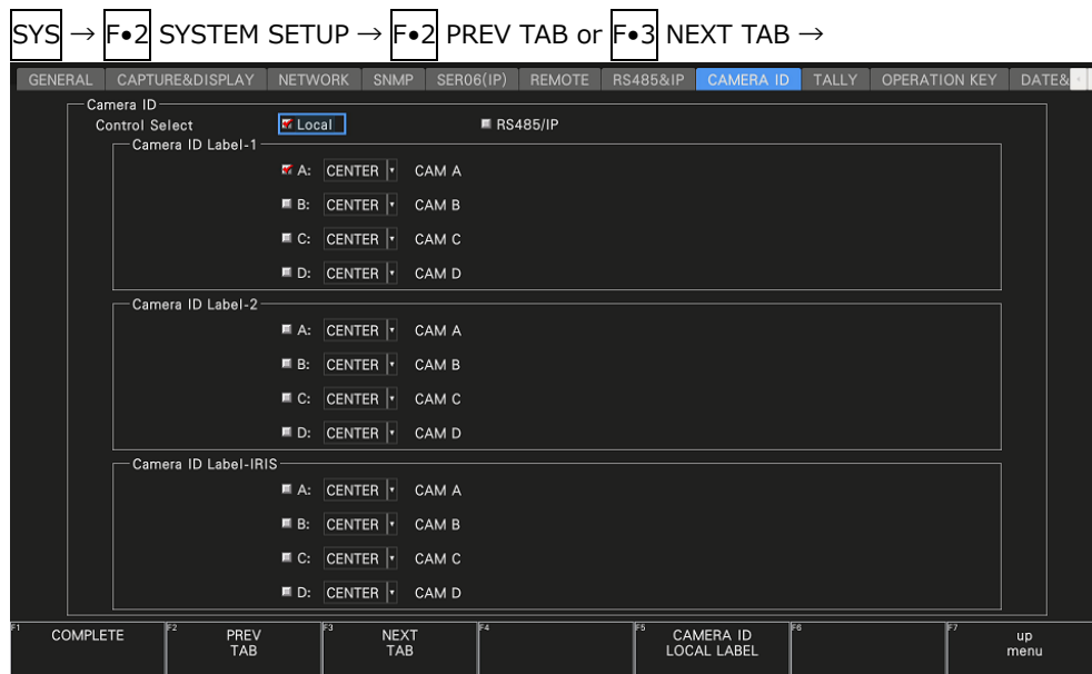
Figure 7-30 CAMERA ID tab
