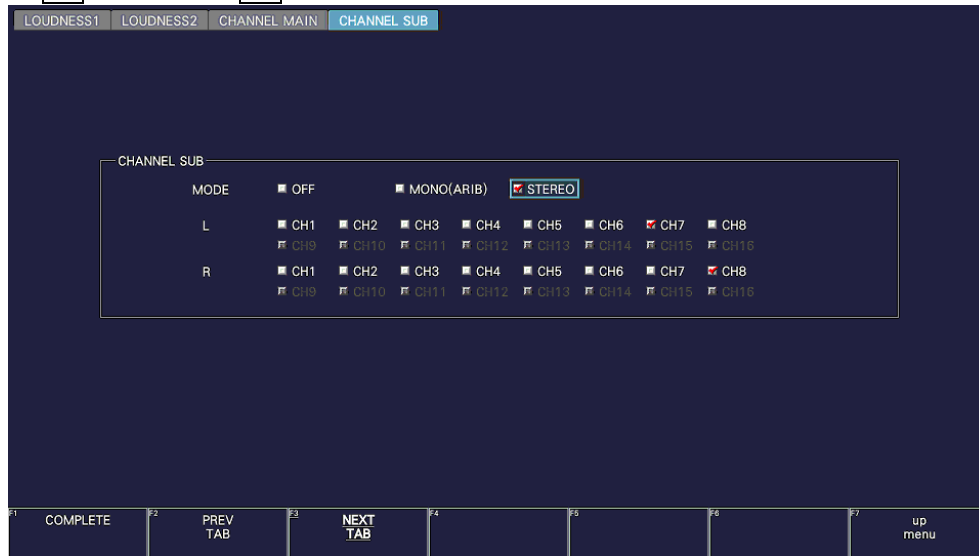
Figure 15-45 CHANNEL SUB tab
