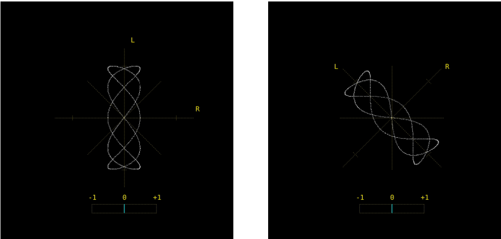
Figure 15-21 Selecting the scale display format
