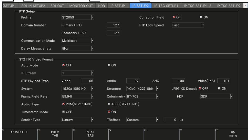
Figure 7-11 IP SETUP2 tab
