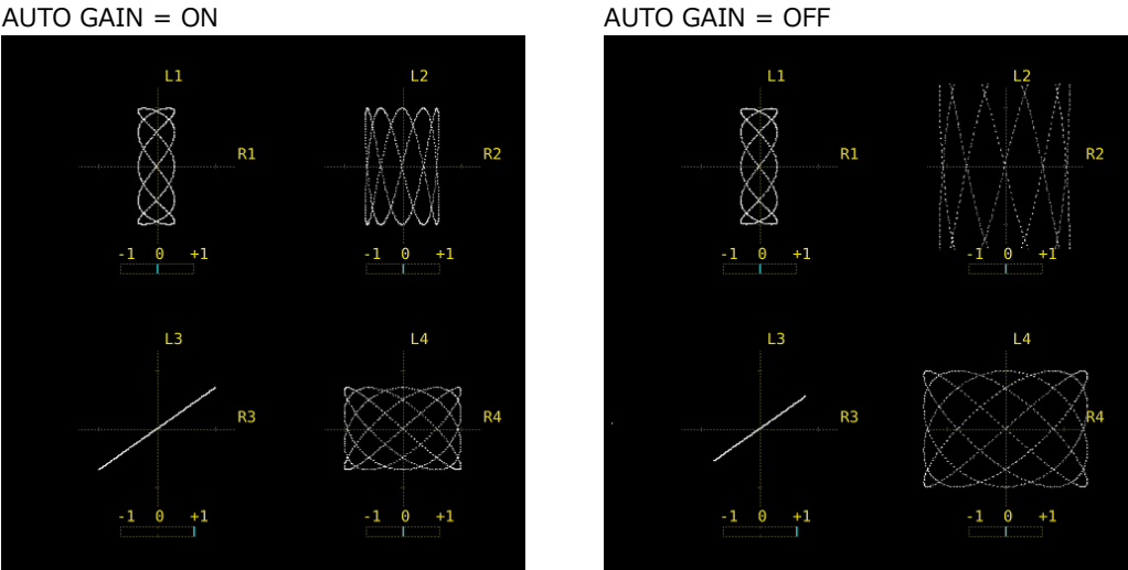
Figure 15-22 Setting the Lissajous curve gain
