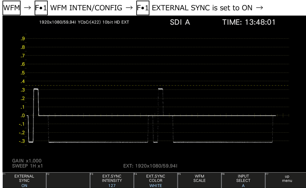
Figure 10-30 EXTERNAL SYNC men
