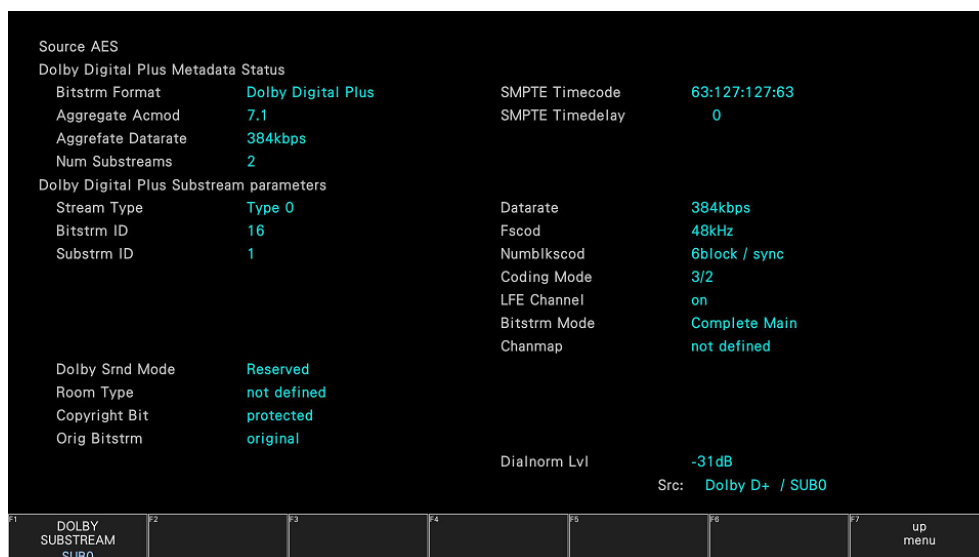
Figure 15-33 Dolby Digital Plus metadata display (SER04)
