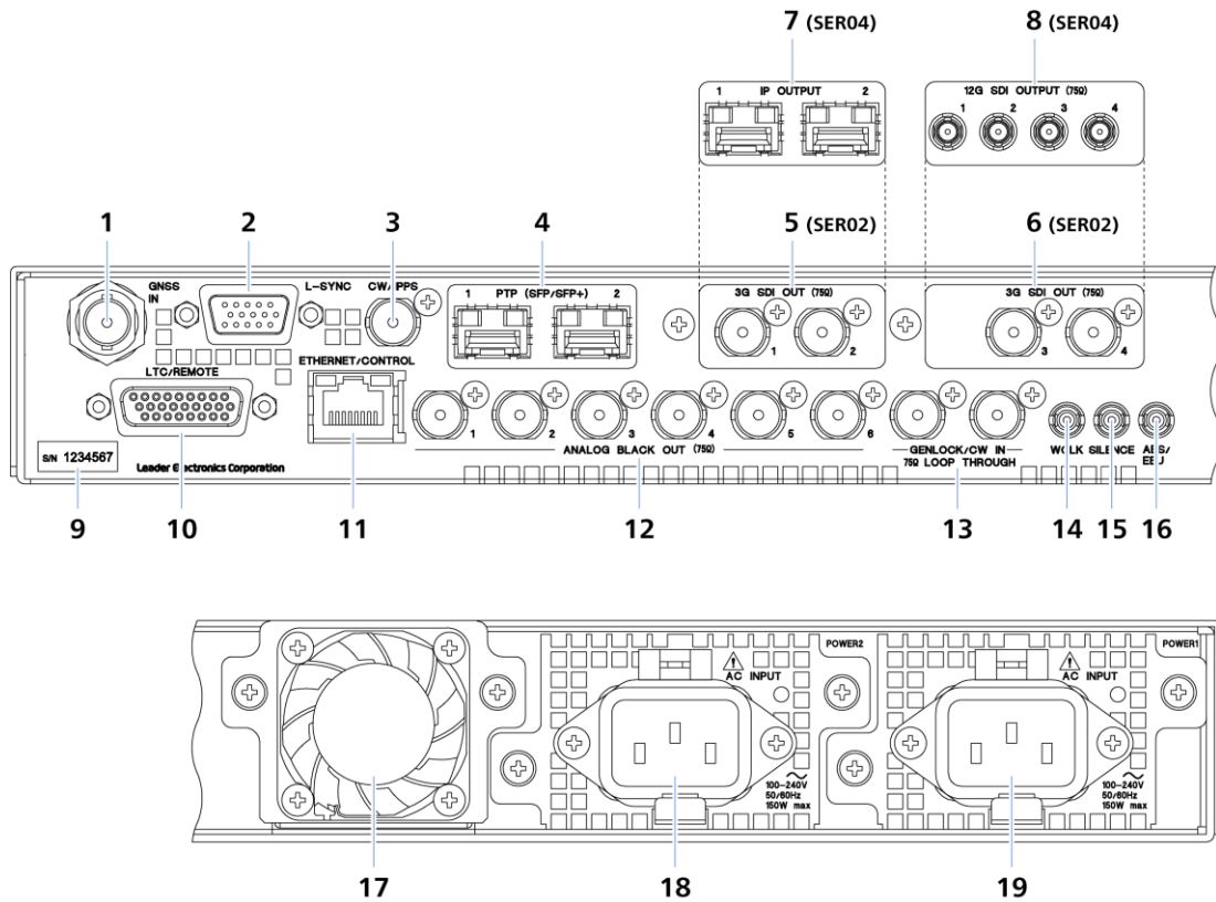
Figure 4-4 | Rear panel (enlarged view)
