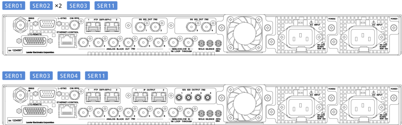
Figure 4-3 | Rear panel (overall view)
